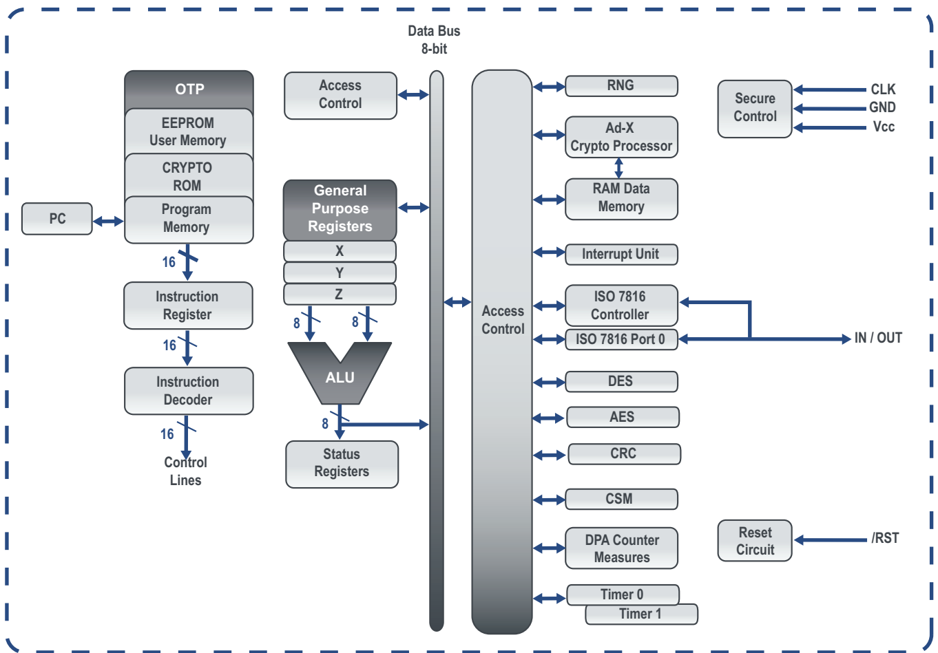
Figure 1 AT90SC4040CV RISC CPU Core Architecture
