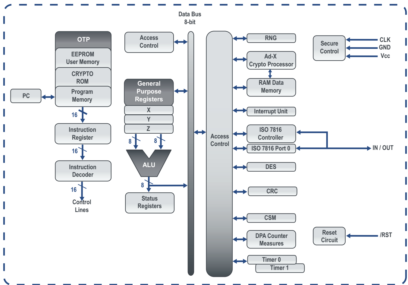
Figure 1 Shows a block diagram of the AT90SC20818RCV
